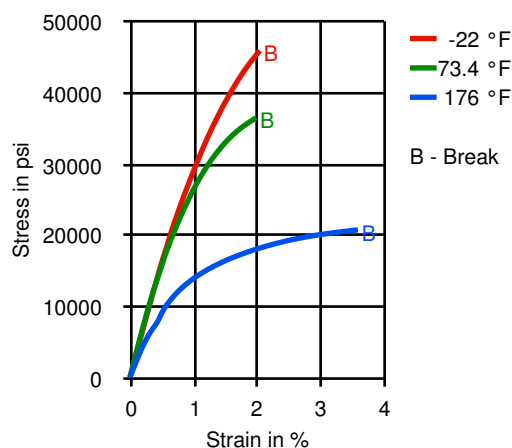
True Stress-strain
