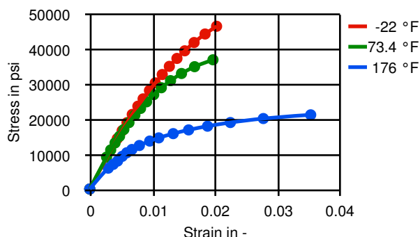
True Stress-strain
