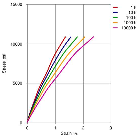
CAMPUS Stress-strain (isochronous) 73.4 °F
