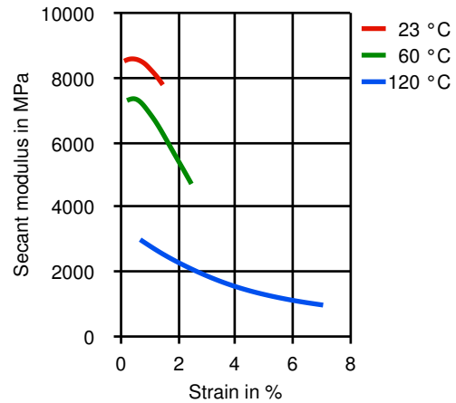
Secant modulus-strain
