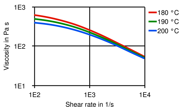
Viscosity-shear rate
