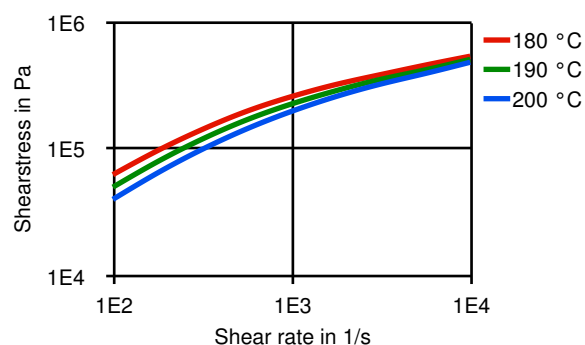
Shearstress-shear rate
