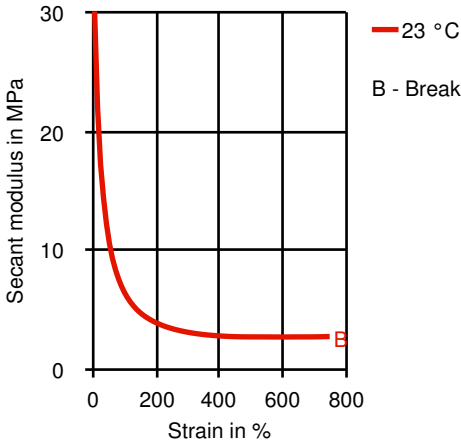
Secant modulus-strain
