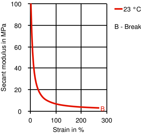
Secant modulus-strain
