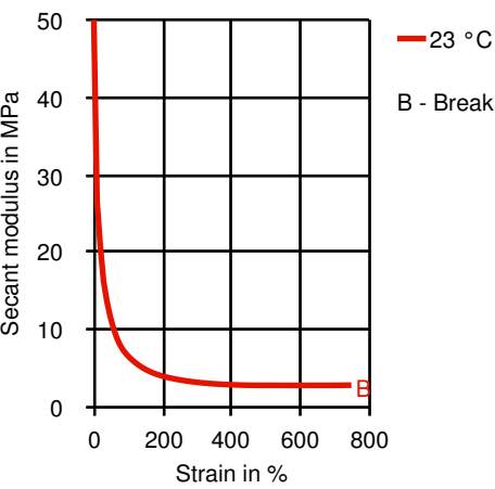
Secant modulus-strain
