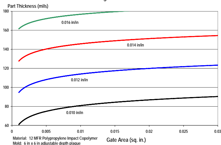
Contour Plots of Constant Mold Shrinkage as a Function of Gate Area and Part Thickness
