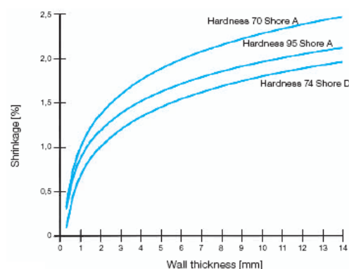
Shrinkage in relation to wall thickness
