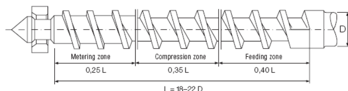
Screw configuration (diagrammatic view)
