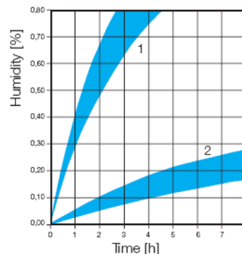
Moisture absorption Polyether-TPU Hardness 80 Shore A – 64 Shore D
