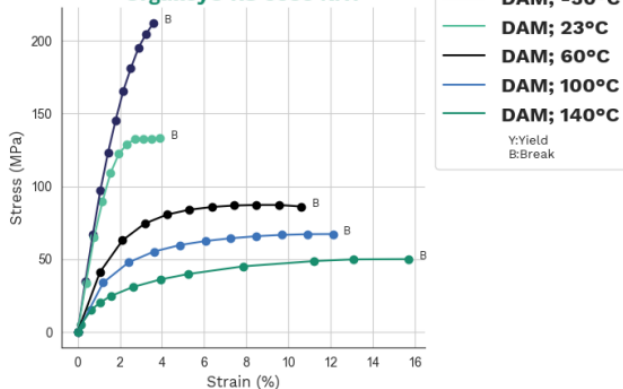
Stress-strain Orgalloy® RS 6030 NAT
