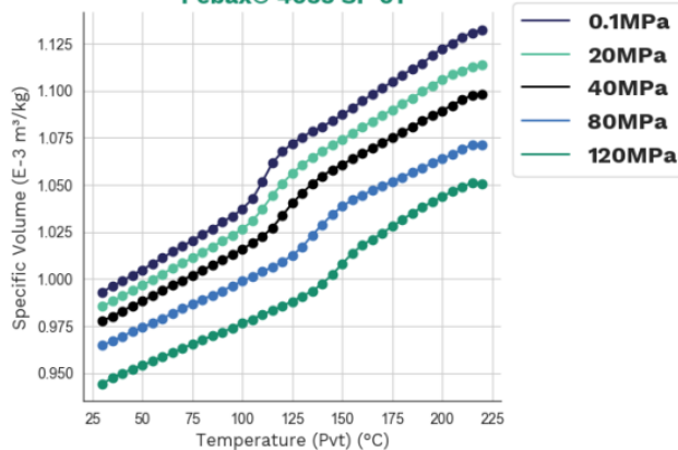
Specific volume-temperature (pvT) Pebax® 4033 SP 01
