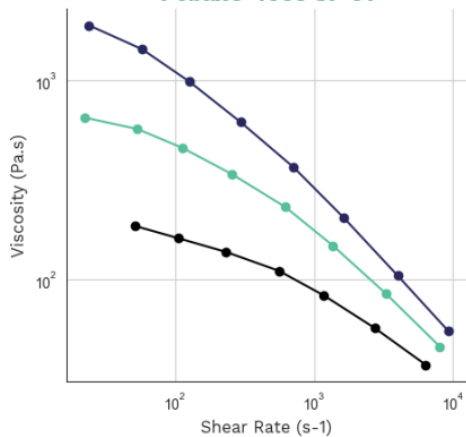
Viscosity-shear rate Pebax® 4033 SP 01
