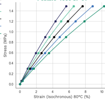
Stress-strain (Isochronous) 80°C Pebax® 4033 SP 01
