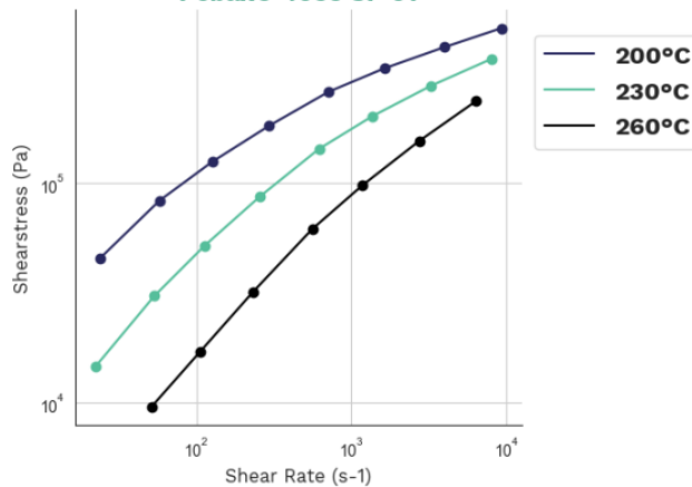
Shearstress-shear rate Pebax® 4033 SP 01
