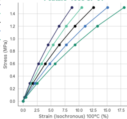
Stress-strain (Isochronous) 100°C Pebax® 4033 SP 01
