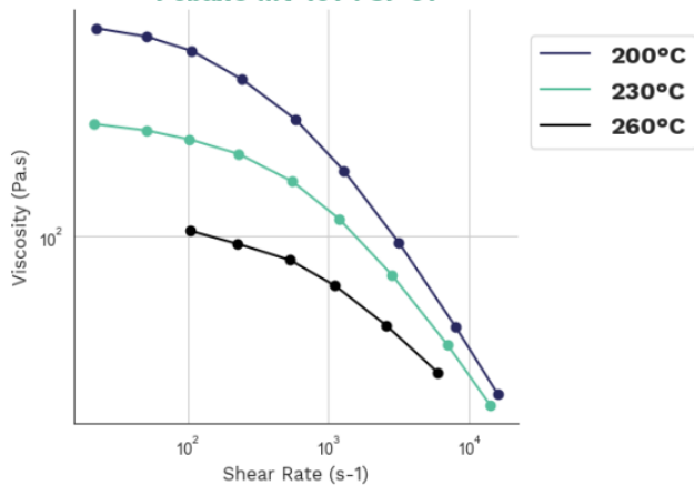
Viscosity-shear rate Pebax® MV 1074 SP 01
