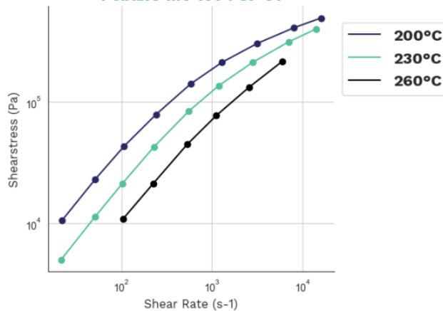
Shearstress-shear rate Pebax® MV 1074 SP 01
