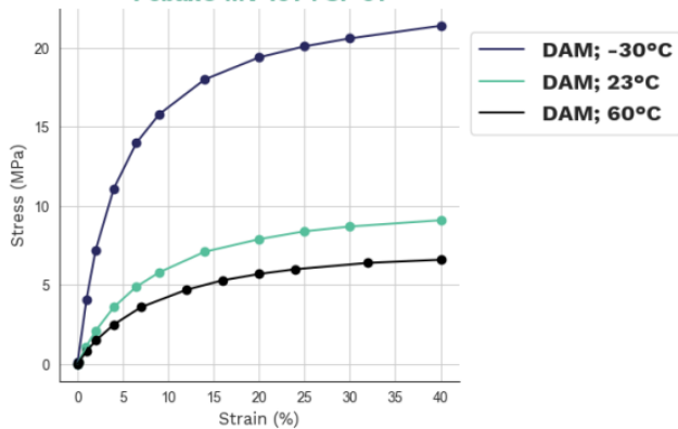
Stress-strain Pebax® MV 1074 SP 01
