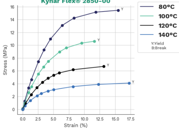
Stress-strain Kynar Flex® 2850-00
