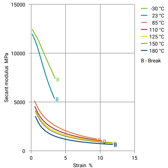
Tensile modulus-temperature (dry)
