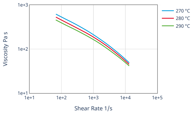
Viscosity-shear rate
