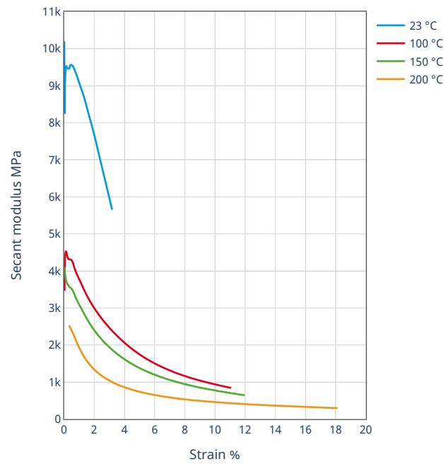
Secant modulus-strain
