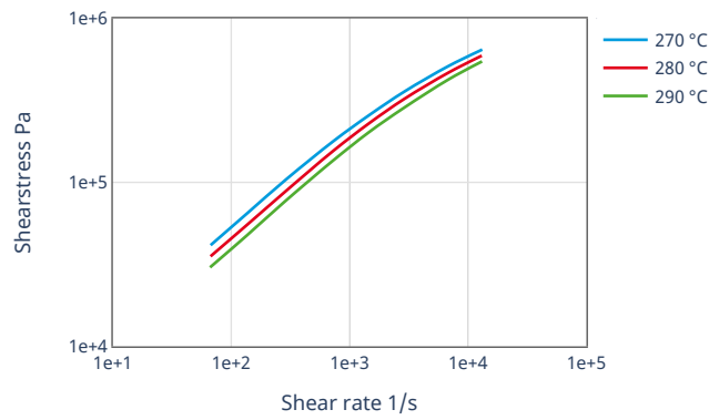
Shearstress-shear rate
