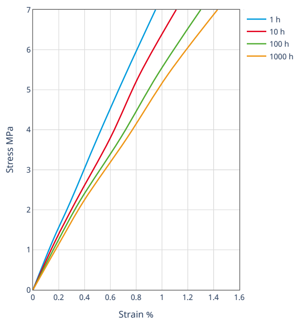
Stress-strain (isochronous) 160°C
