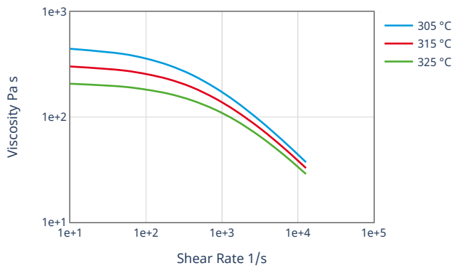
Viscosity-shear rate
