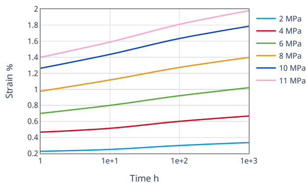
Creep curve 100°C
