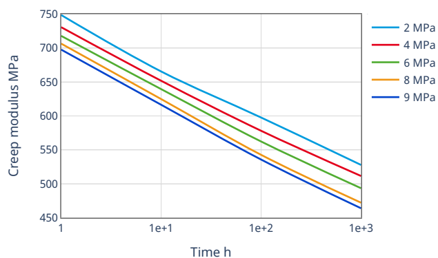
Creep modulus-time 140°C
