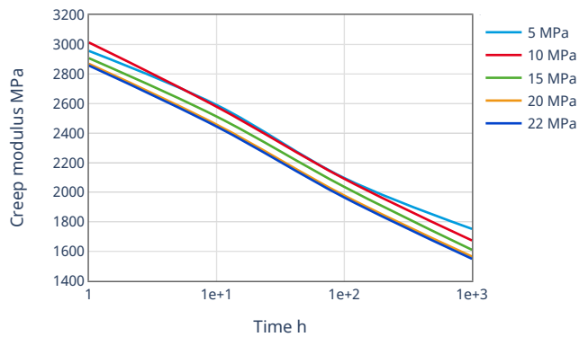
Creep modulus-time 23°C
