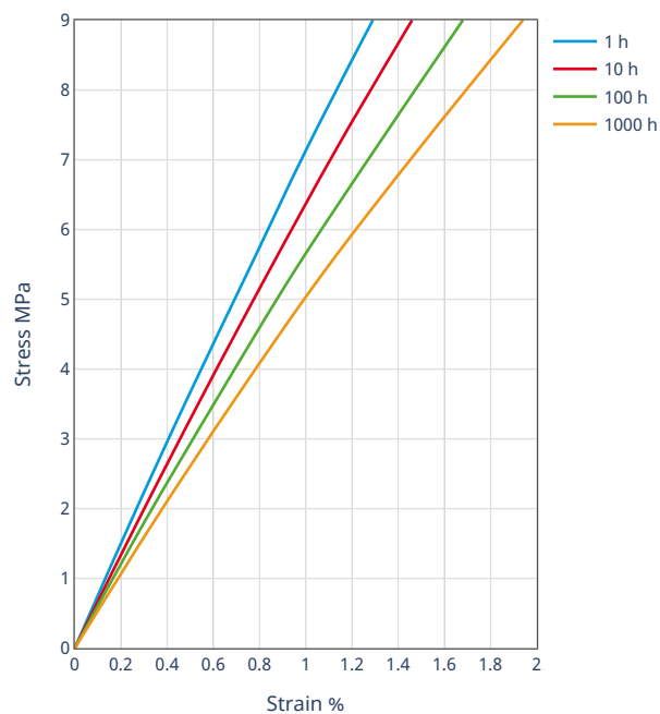
Stress-strain (isochronous) 140°C
