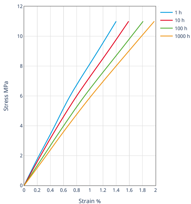
Stress-strain (isochronous) 100°C
