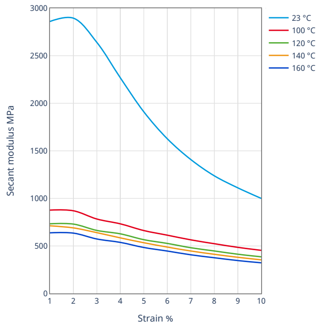
Secant modulus-strain
