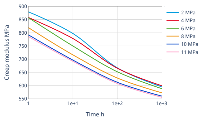
Creep modulus-time 100°C
