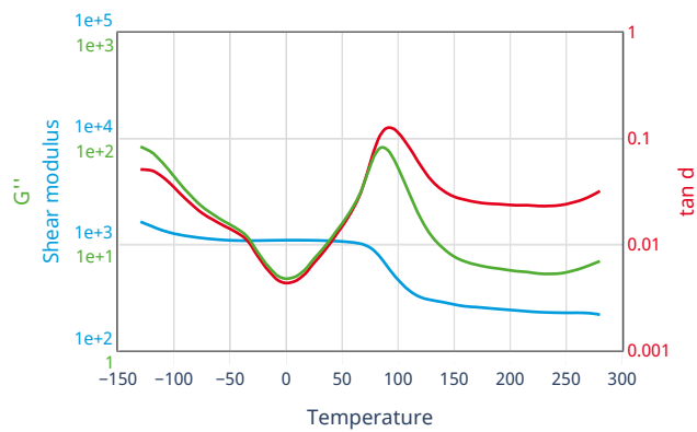
Dynamic shear modulus-temperature
