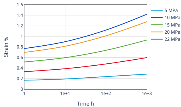
Creep curve 23°C
