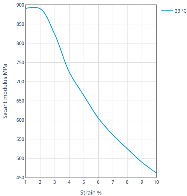
Secant modulus-strain
