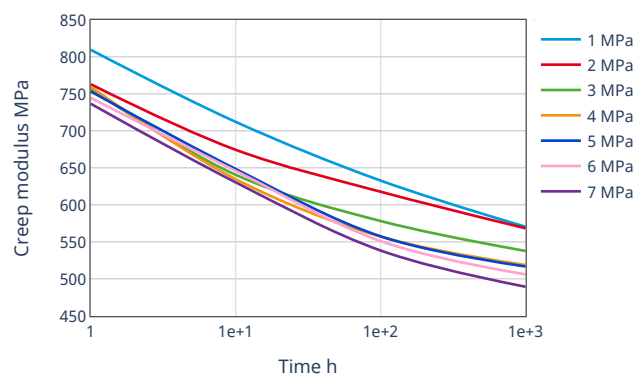
Creep modulus-time 160°C
