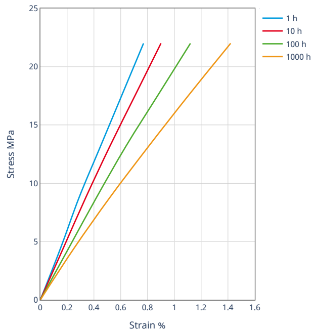
Stress-strain (isochronous) 23°C
