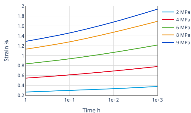
Creep curve 140°C
