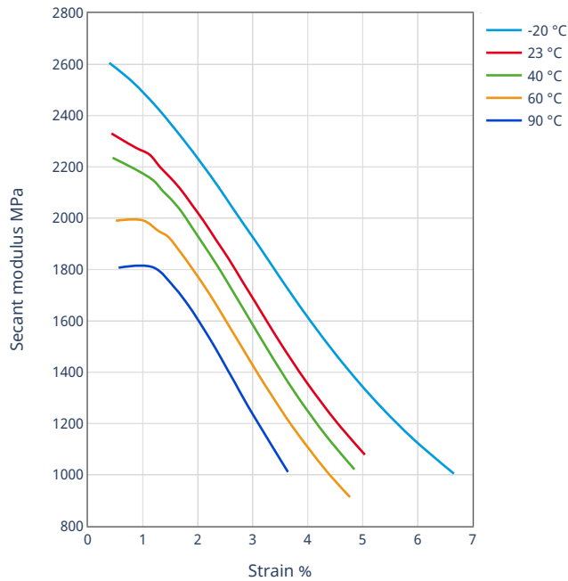
Secant modulus-strain
