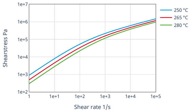
Shearstress-shear rate
