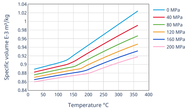
Spec. volume-Temperature (pVT)
