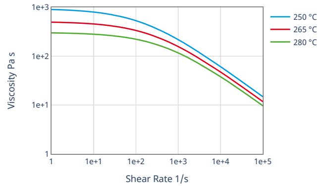
Viscosity-shear rate
