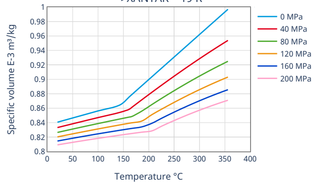
Spec. volume-Temperature (pVT) ->XANTAR™ 19 R
