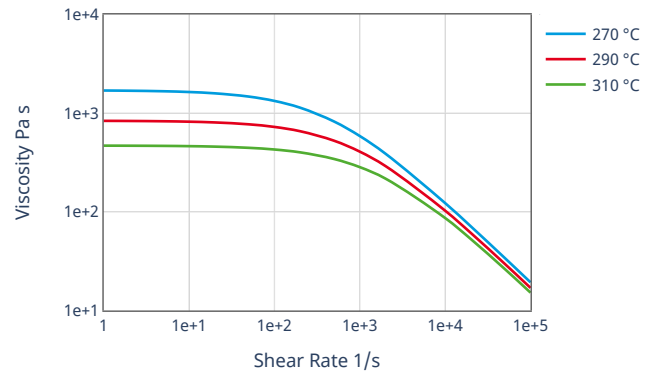
Viscosity-shear rate
