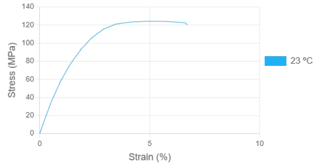
Stress-strain, conditioned
