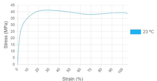
Stress-strain, conditioned
