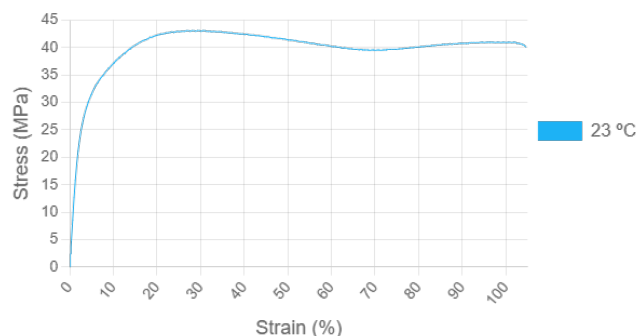
Stress-strain, conditioned
